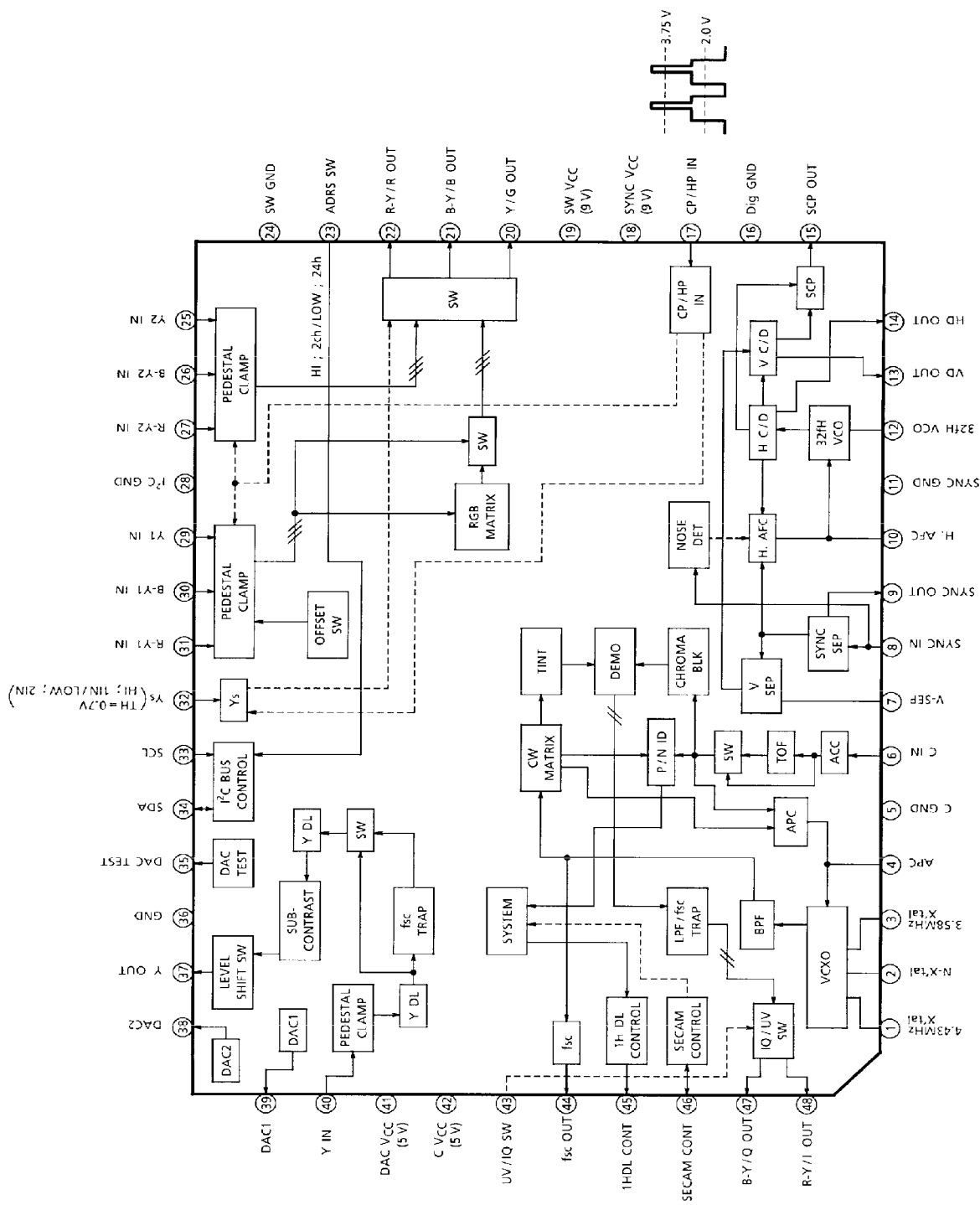
BLOCK DIAGRAM
