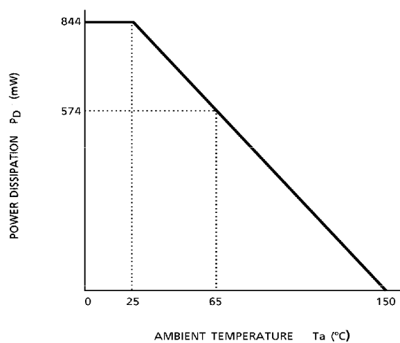
Fig. Power dissipation temperature reduction curve
