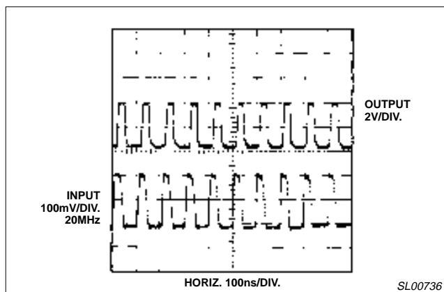
Figure 10. Line Receiver Response
