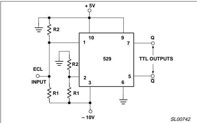
Figure 16. ECL-to-TTL Translator
