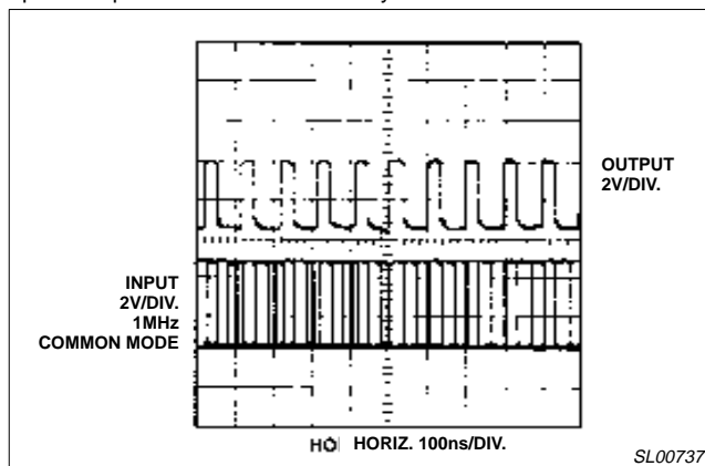
Figure 11. Response During Common-Mode Noise
