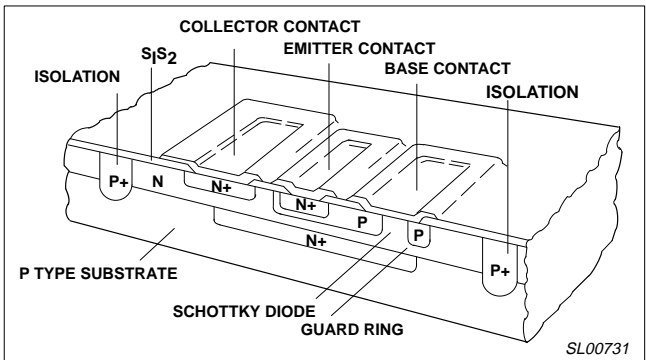
Figure 5. Schottky Clamped Transistor Geometry
