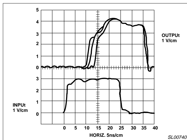
Figure 14. Parallel A/D Response
