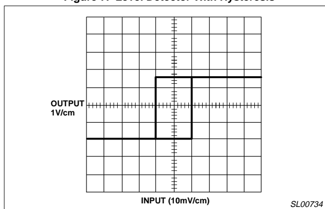
Figure 8. 0V Level Detector With \pm 10\text{mV} Hysteresis Line Receiver
