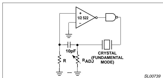
Figure 13. Crystal Oscillator
